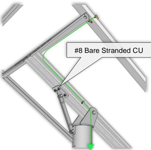
Single Panel GND Wire Route
