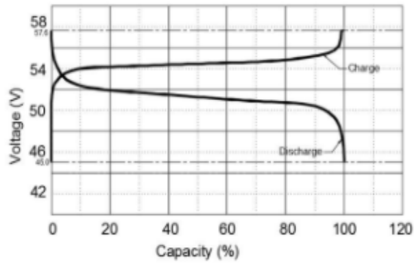
Charge & Discharge curve with 0.5C @ 25°C
