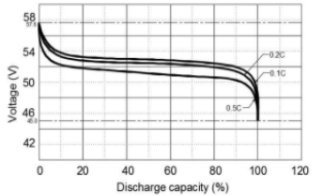
Discharge performance with different rate @ 25°C
