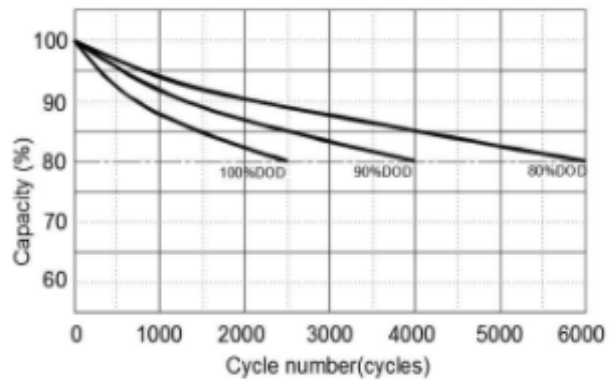
Cycle life with DOD @ 0.5C, 25°C
