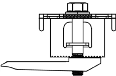
END CLAMP ASSEMBLY
